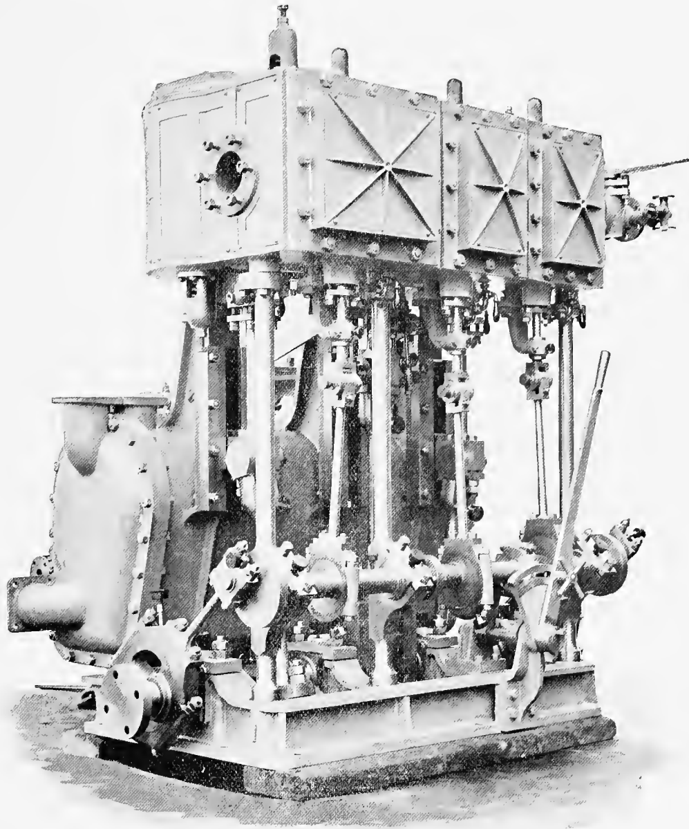
TRIPLE-EXPANSION ENGINE.—Designed and Built by P. Smit, Jr., Rotterdam.
